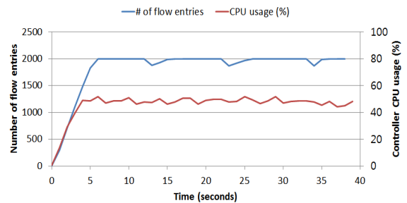
Fig. 1. Before applying the defense mechanism against the resource consumption attacks
