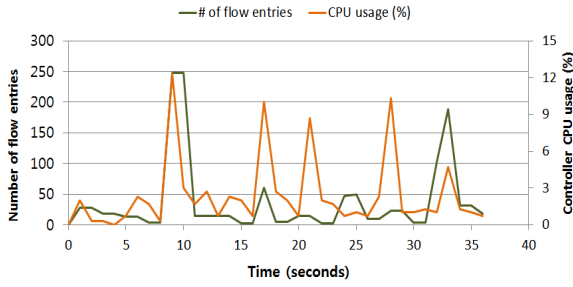
Fig. 2. After applying the defense mechanism against the resource consumption attacks
