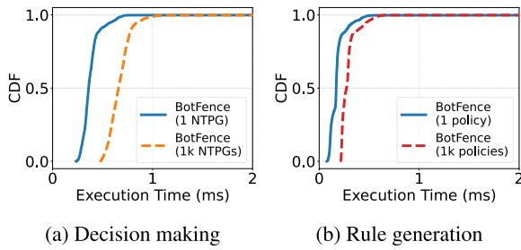
FIGURE 15. (a) Decision making time comparison with the increasing number of NTPGs. (b) Rule generation time comparison with the increasing number of policies.
