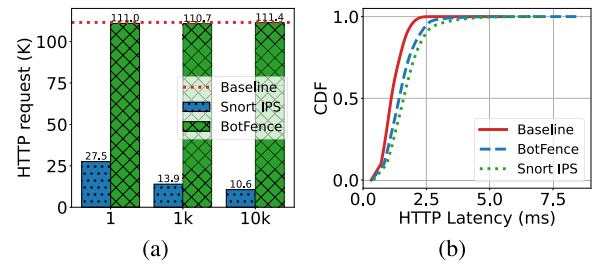
FIGURE 16. (a) L7 throughput comparison with the increasing number of network rules. (b) L7 latency comparison.
