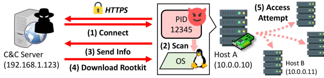
FIGURE 9. A security evaluation scenario consisting of 5 stages. The infiltrated malware in the Host A and attempted to establish communication with the C&C server. To obfuscate its actions, the attacker leveraged an encrypted session.
