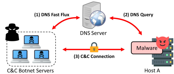
FIGURE 2. Example scenario of C&C session establishment in botnet attack. The attacker hide its IP address by DNS fast flux and encrypt C&C message.
