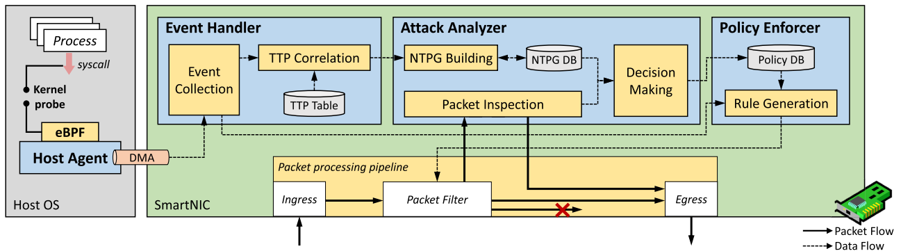
FIGURE 3. The overall architecture and workflow of BotFence with four key components: (i) Host Agent, (ii) Event Handler, (ii) Attack Analyzer, and (iv) Policy Enforcer.
