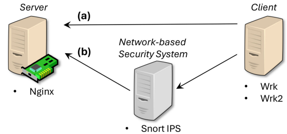
FIGURE 14. Test environments for performance evaluation; BotFence is deployed on the server machine. The route (a) is configured for BotFence, and the route (b) is for Snort IPS.
