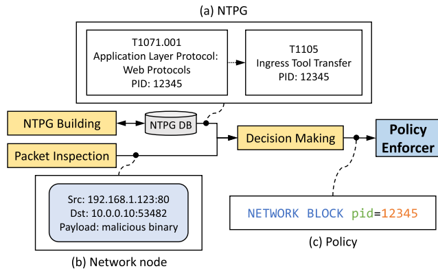
FIGURE 6. The generation of the policy based on constructed NTPG and inspected network information.
