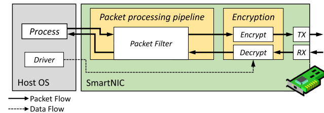
FIGURE 7. BotFence utilizes encryption module to offload packet encryption to the SmartNIC for packet inspection.
