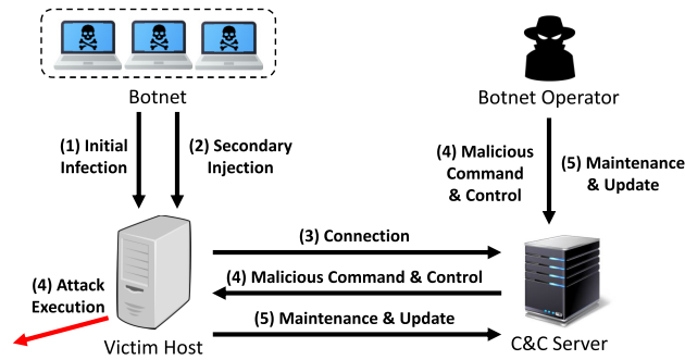
FIGURE 1. Lifecycle of Botnet.
