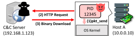
FIGURE 4. The botnet malware installed in the host tries to connect C&C server via HTTP protocol.
