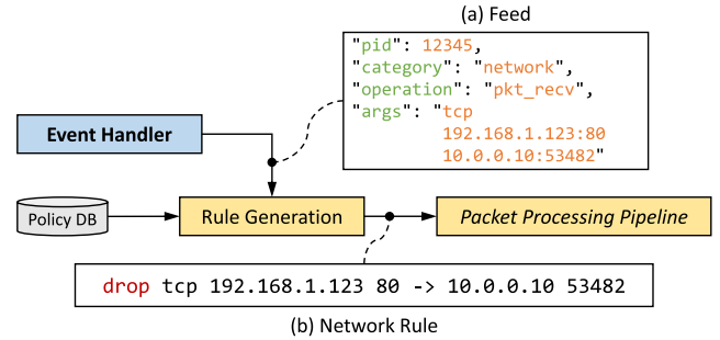
FIGURE 8. The generation of network rule by the network feed of the process which violates deployed policy.
