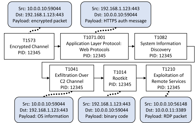
FIGURE 12. Network enhanced TTP Provenance Graph (NTPG) related to the attack scenario (Figure 9).
