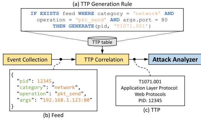
FIGURE 5. The transformation of the host event received from the agent into a TTP.
