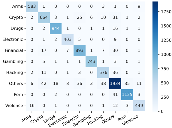
(c) DarkBERT raw
