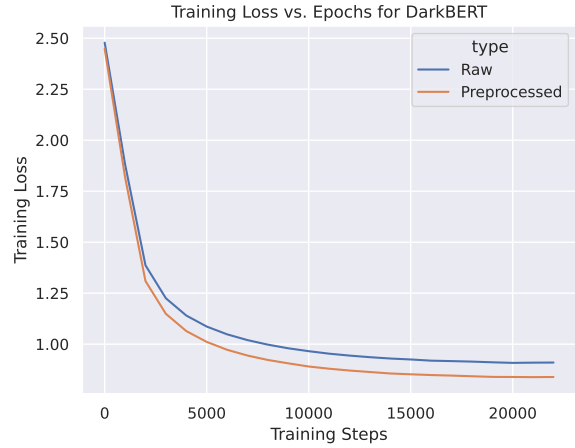
Figure 2: Training steps vs. training loss graph for raw and preprocessed versions of DarkBERT.
