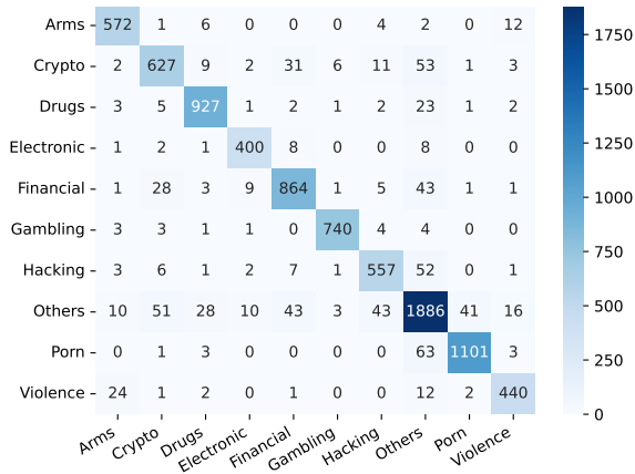
(a) BERT cased
