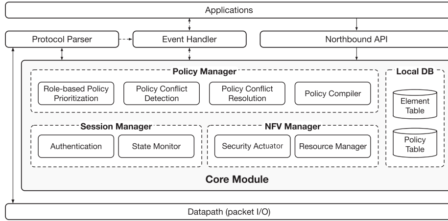
Fig. 4. The internal composition of the core module.
