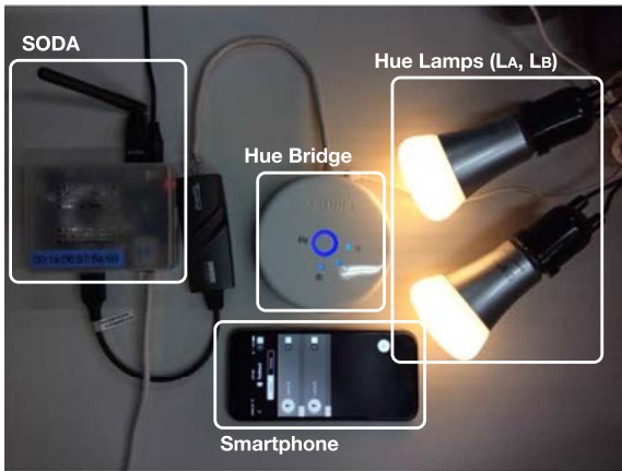
Fig. 10. Test environment with SODA and real IoT devices.
