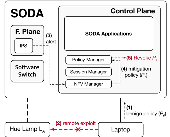
Fig. 12. Operation scenario for remote exploit detection.
