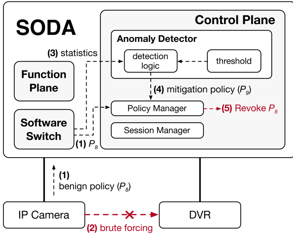
Fig. 13. Operation scenario for botnet mitigation.
