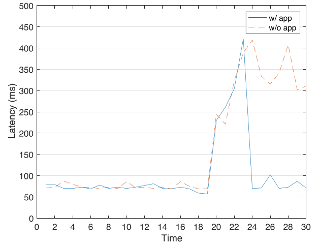
Fig. 14. Inter-device latency variations during a DoS attack.
