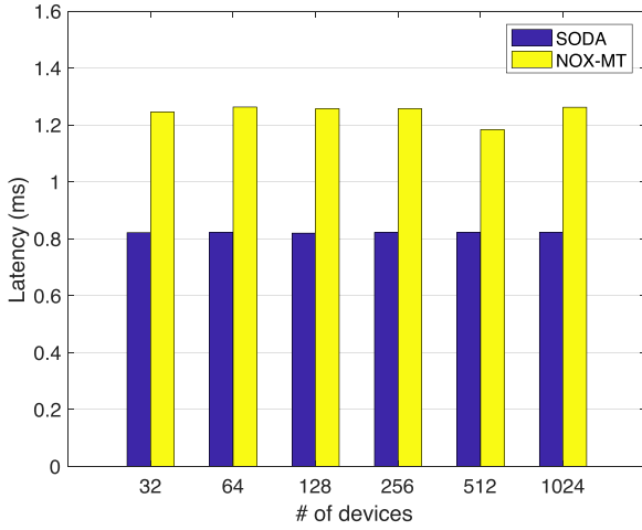
Fig. 9. Latency comparison of SODA with NOX-MT.
