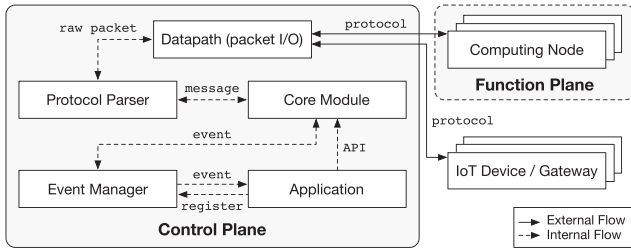
Fig. 2. The overall architecture of SODA.
