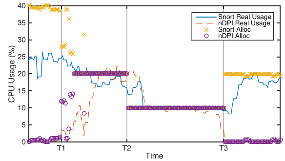
Fig. 15. Resource management in the function plane.
