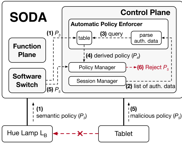
Fig. 11. Operation scenario for automatic policy enforcer.
