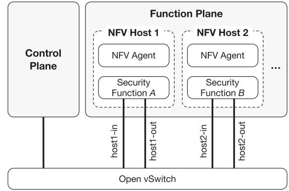
Fig. 5. The implementation diagram of SODA's prototype.
