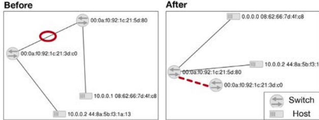
Fig. 16. Results of the Link-Discovery-Neutralization attack experiment. A circle (before) represents a live link between two switches, and a dotted line (after) represents a failed link.
