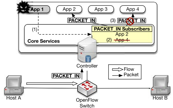
Fig. 2. Event Listener Unsubscription attack.
