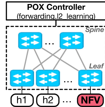
Fig. 27. Leaf-spine topology.
