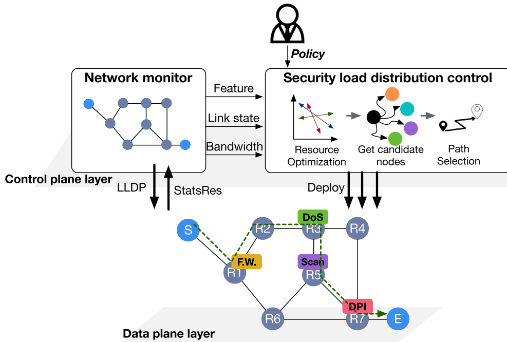
Fig. 15. Workflow of resource-aware action deployment.
