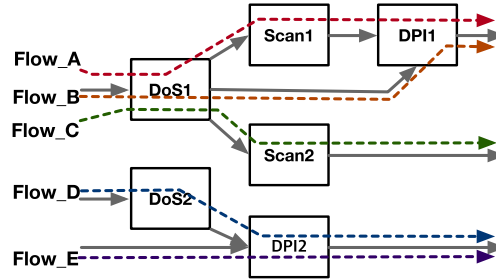
(a) An example of security service chains on NfV nodes.
