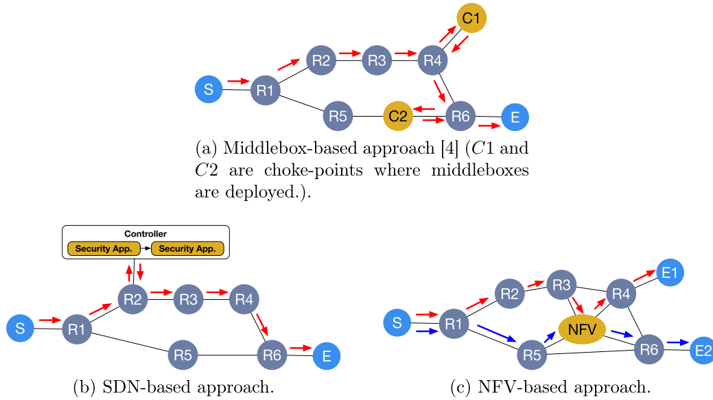
Fig. 1. The illustration of deployment strategies for security solutions in a dynamic network. S and E denote a source and destination respectively. R^* denotes network devices (i.e., routers or switches).
