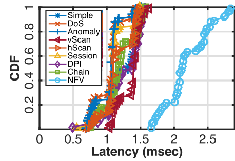
Fig. 21. Latency of the software-based DPX.
