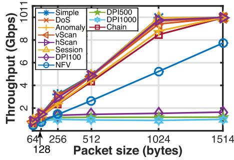
Fig. 20. Throughput of the software-based DPX.
