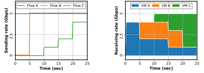
Fig. 11: Bandwidth reservation
