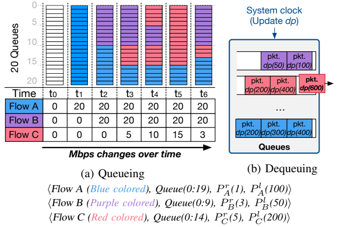
Fig. 5: Operation example of MECaNIC queueing system
