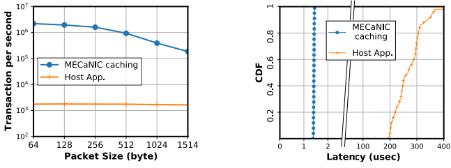
(a) TPS for packet transfer (b) Session establishment time elapsed Fig. 13: TCP session-packet transferring
