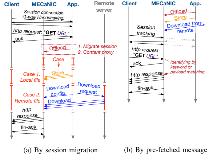
Fig. 7: Example of the response caching for HTTP
