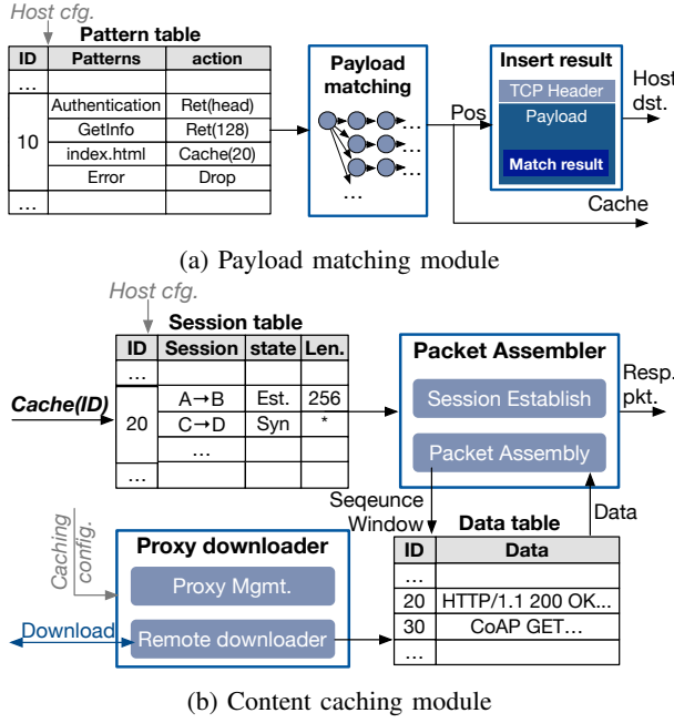
Fig. 6: Design of task offloading module
