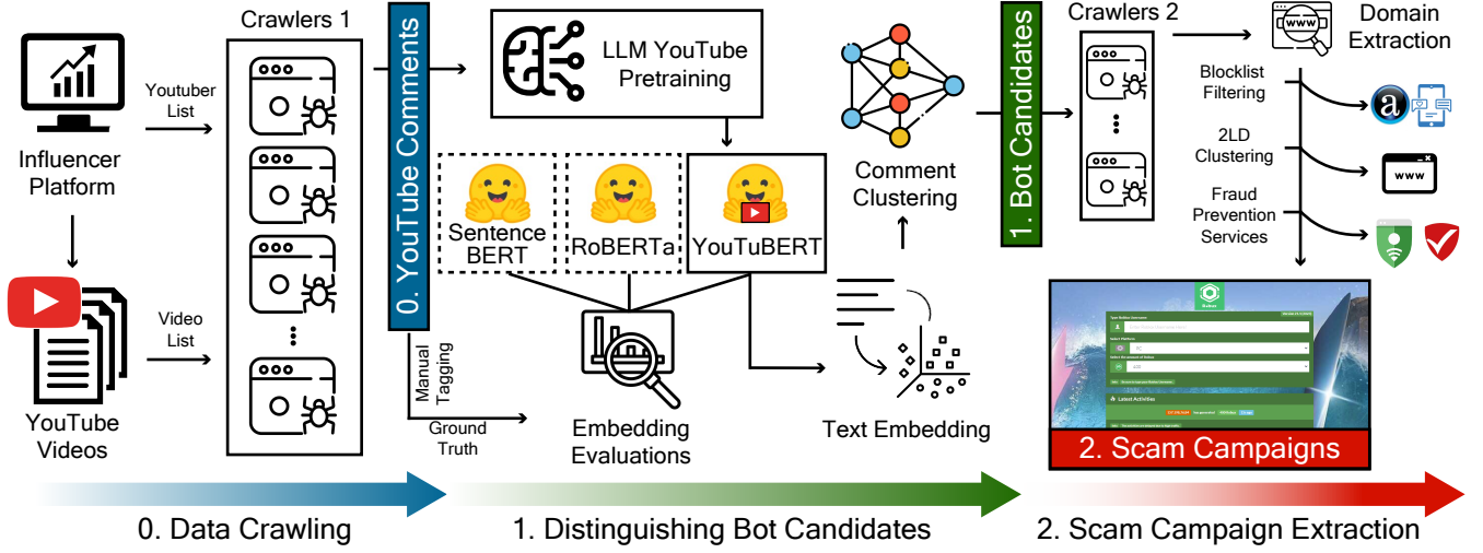
Figure 3: Workflow to extract SSBs and their scam campaigns. The output is colored to match its respective phase.
