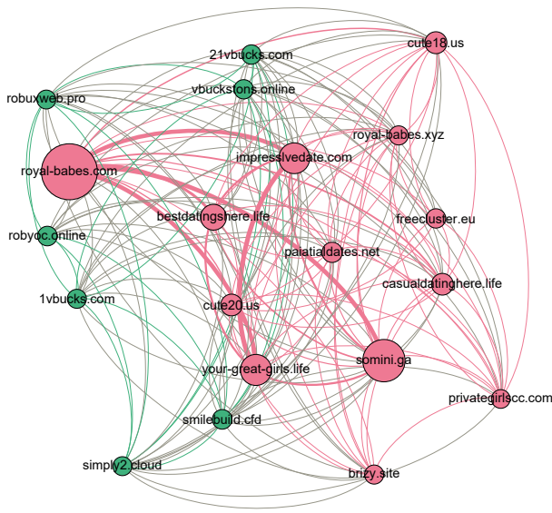
Figure 7: Top 20 scam campaign graph based on video infections. Campaigns are connected by the number of overlapping videos (edge width) in which they infect. Node size represents the number of SSBs in control.
