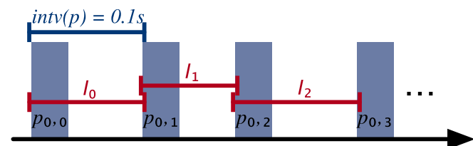
Fig. 14. Definitions for measuring time precision.
