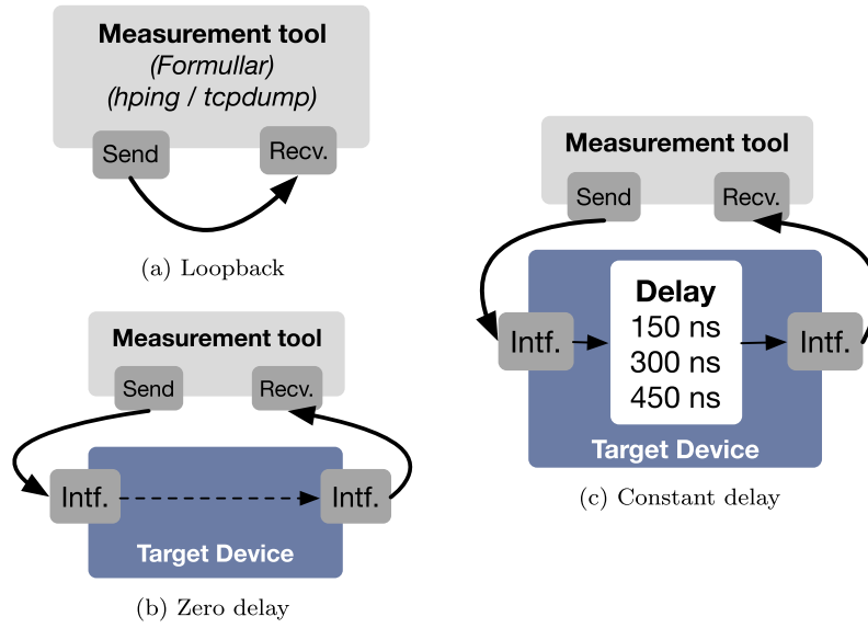
Fig. 10. Evaluation setup.
