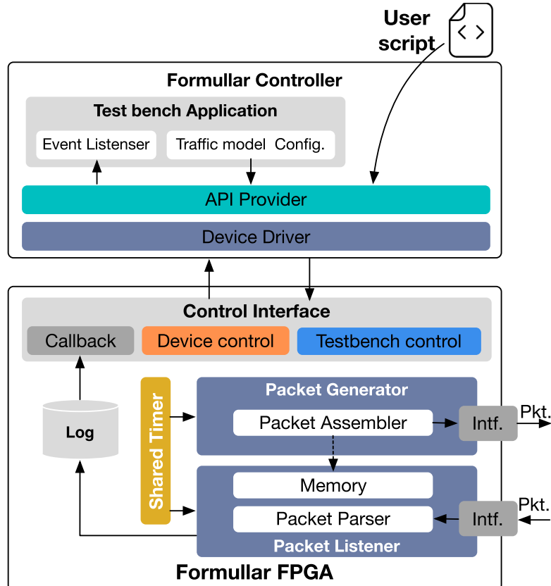
Fig. 3. Formullar architecture.
