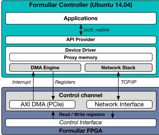
Fig. 8. Controller implementation details.
