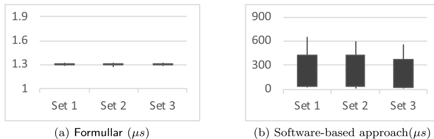
Fig. 12. Results for the no-delay case.
