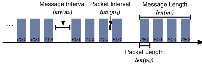
Fig. 2. Traffic model.
