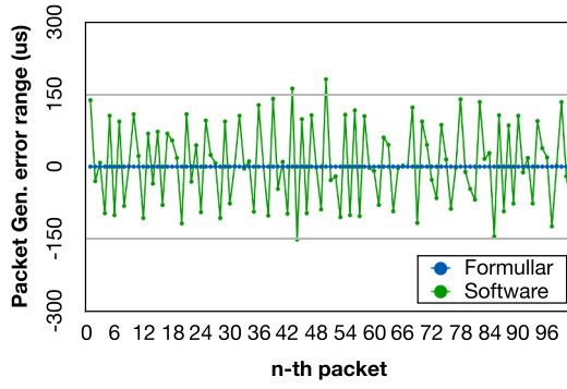
(a) Packet generation time deviation
