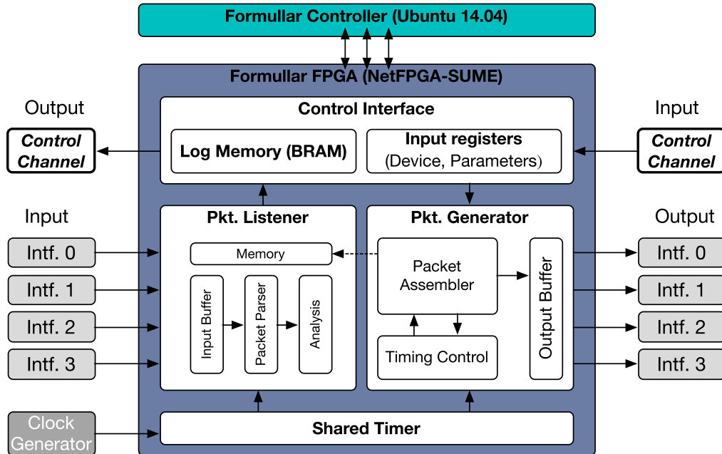
Fig. 7. FPGA implementation details.
