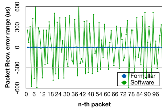
(b) Packet receipt time deviation
