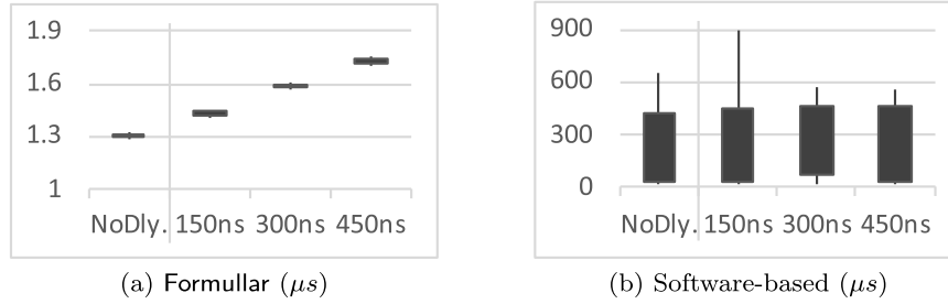
Fig. 13. Results for the constant delay cases.
