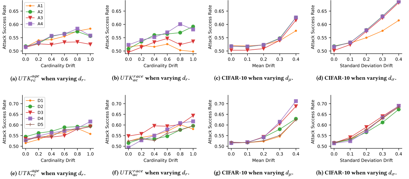
Figure 2: The change in MIA success rate when varying the degree of data drift in multiple scenarios. The upper graphs compare the attacks in the defense setting of early stopping (D1) and the lower graphs compare the defense methods in the attack setting of MIA based on prediction modified entropy (A4). Graphs on the rest of the cases can be found in link.
