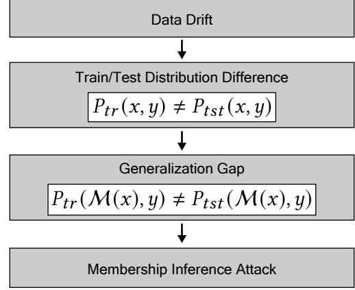
Figure 1: How data drift affects membership inference attacks. Data drift scenarios will lead to a generalization gap in the model, making it prone to membership inference attacks.
