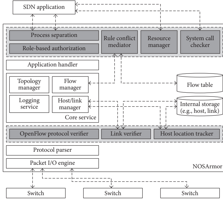
FIGURE 2: High-level overview of NOSArmor architecture.
