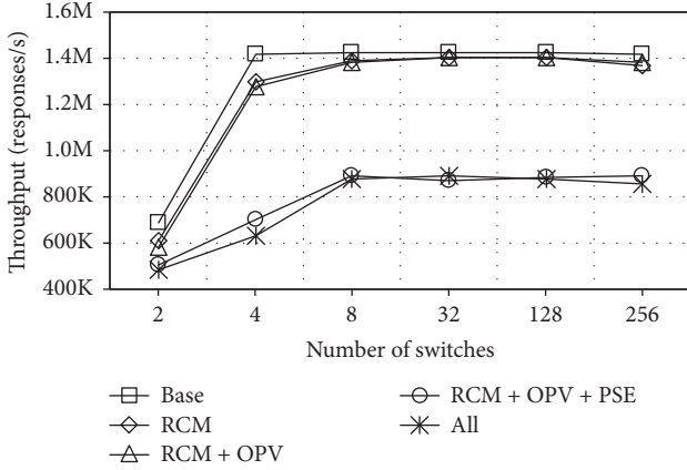
FIGURE 18: Throughput comparison according to combination of SBBs. Note. RCM: Rule Conflict Mediator, OPV: OpenFlow Protocol Verifier, and PSE: Process Separation.
