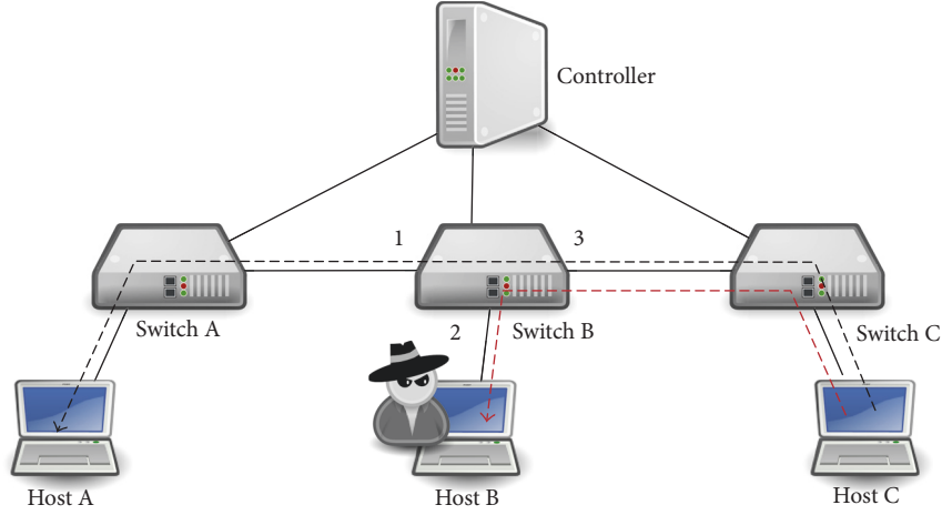
FIGURE 8: Test environment for evaluating the effectiveness of host location tracker.
