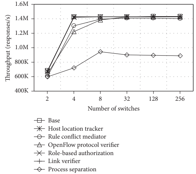
FIGURE 17: Throughput comparison between a base controller and SBBs.
