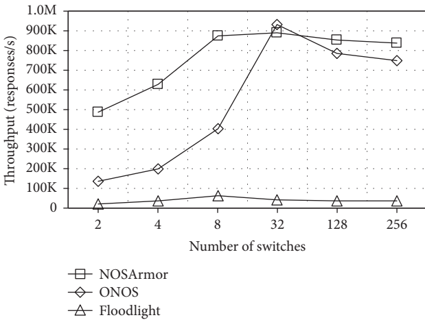
FIGURE 19: Throughput comparison between NOSArmor, ONOS, and Floodlight.
