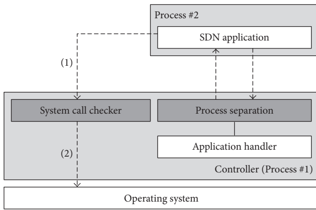
FIGURE 5: System call checker operating scenario.
