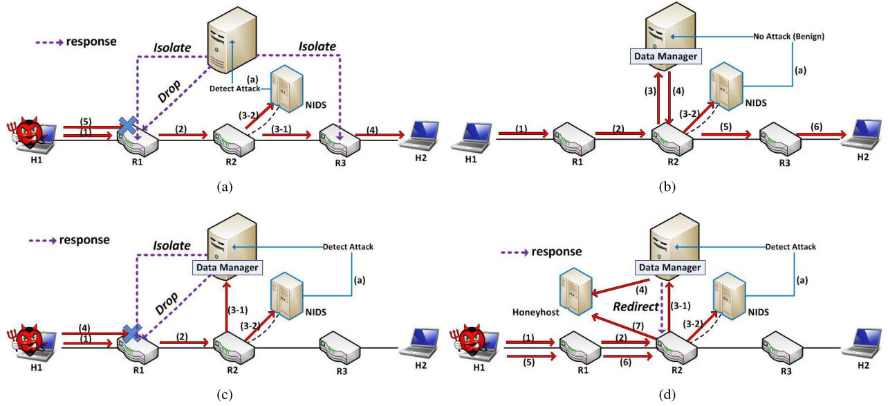
Fig. 4. Response Strategies. (a) Passive Mode Drop/Isolate (attack). (b) In-line mode Forward (benign). (c) In-line mode Drop/Isolate (attack). (d) In-line mode Redirect (attack).
