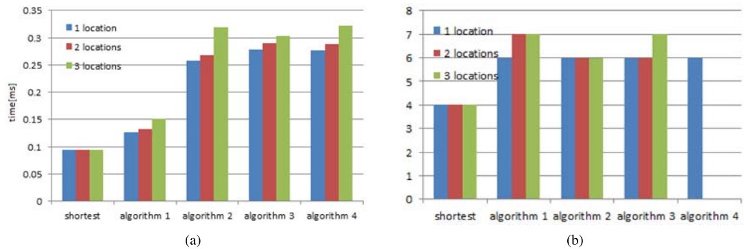
Fig. 8. 6-router topology. (a) Generation Time Measurement. (b) Network Cost Measurement.
