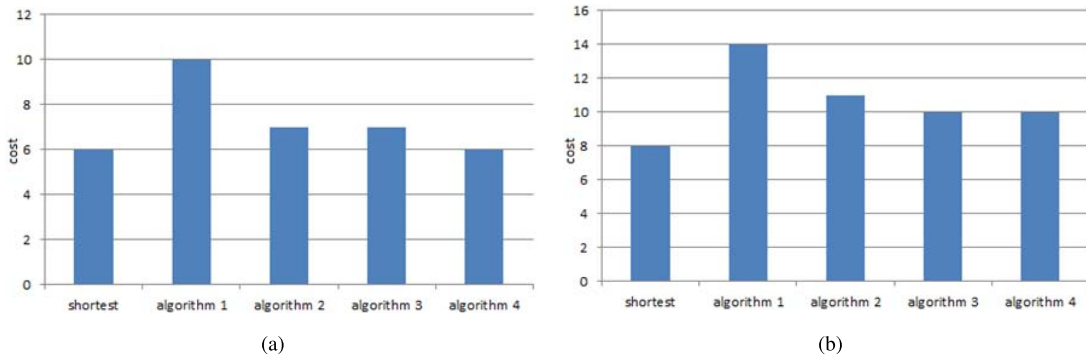
Fig. 7. Network Cost Measurement. (a) 12 routers. (b) 64 routers.
