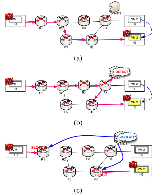
Fig. 1. Example scenario to show how NETSECVISOR works. R (R1, R2, ..., R6) denotes a network router. H (H1, H2, H3) denotes a host (computer). VM (VM1, VM2) denotes a virtual machine. NIDS denotes a network intrusion detection system. And, the devil icon denotes a compromised virtual machine. (a) NIDS missing attack packets (w/o NETSECVISOR). (b) Redirecting attack packets to NIDS (w NETSECVISOR). (c) Isolating compromised VMs (w NETSECVISOR).
