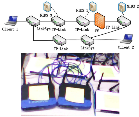
Fig. 5. 6-router Testbed.
