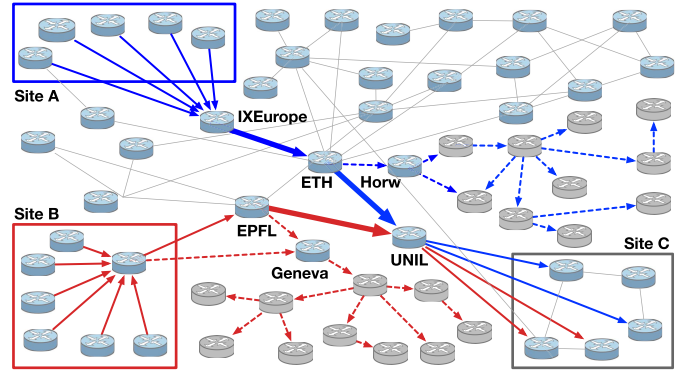
Fig. 13. The SWITCH topology used for testing dynamic metric reduction. The blue and red arrows denote attack flows sent from Site A and B to Site C, respectively. The dashed lines indicated rerouted flows and the grey nodes represent deployed virtual nodes.
