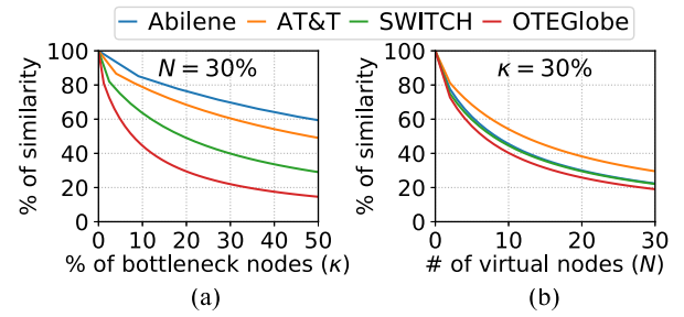
Fig. 10. Measured topology similarity for variants of \kappa and N .
